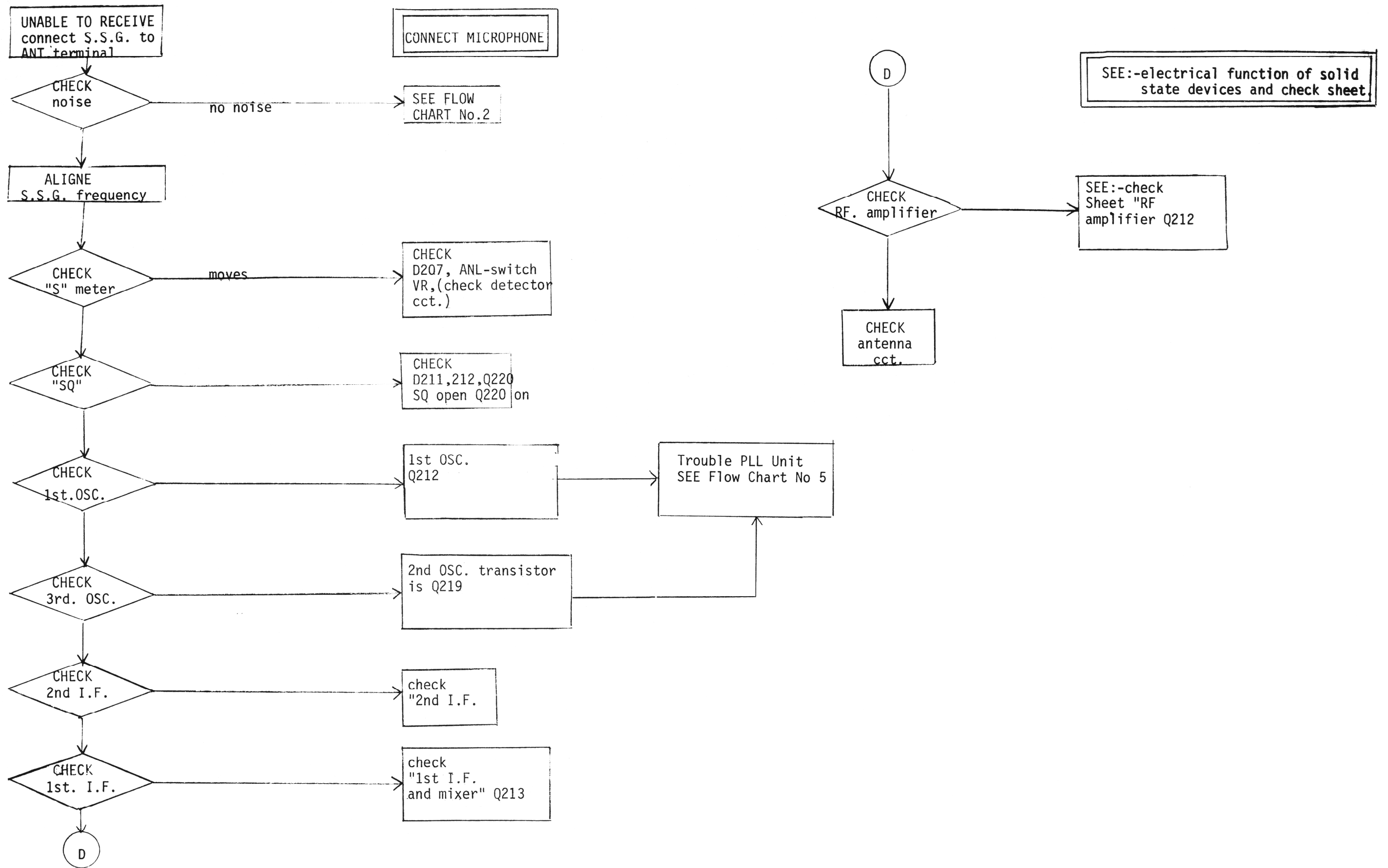
RECEIVER CIRCUIT FLOW CHART NO.3
