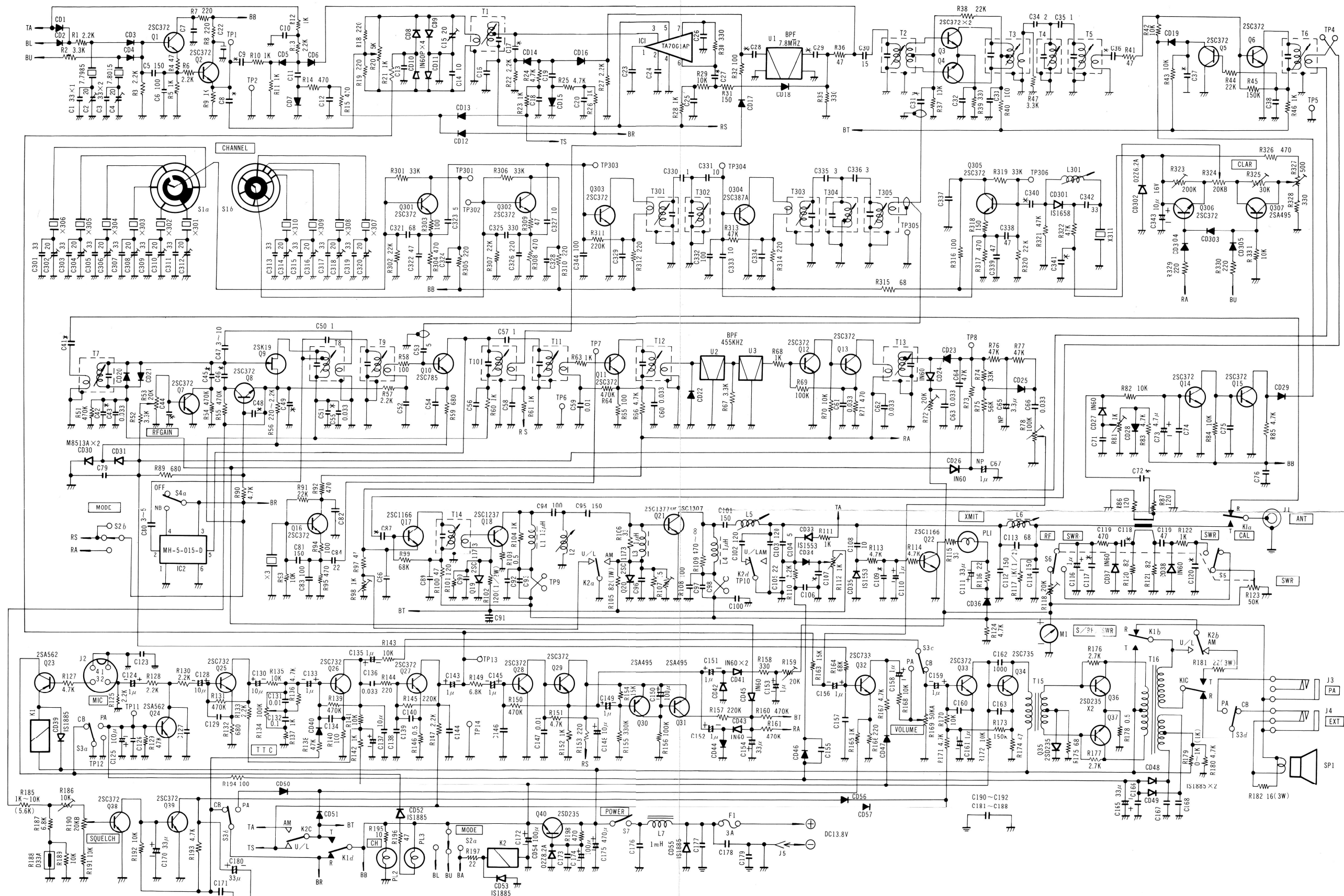
SCHEMATIC DIAGRAM OF DIAMOND 60
