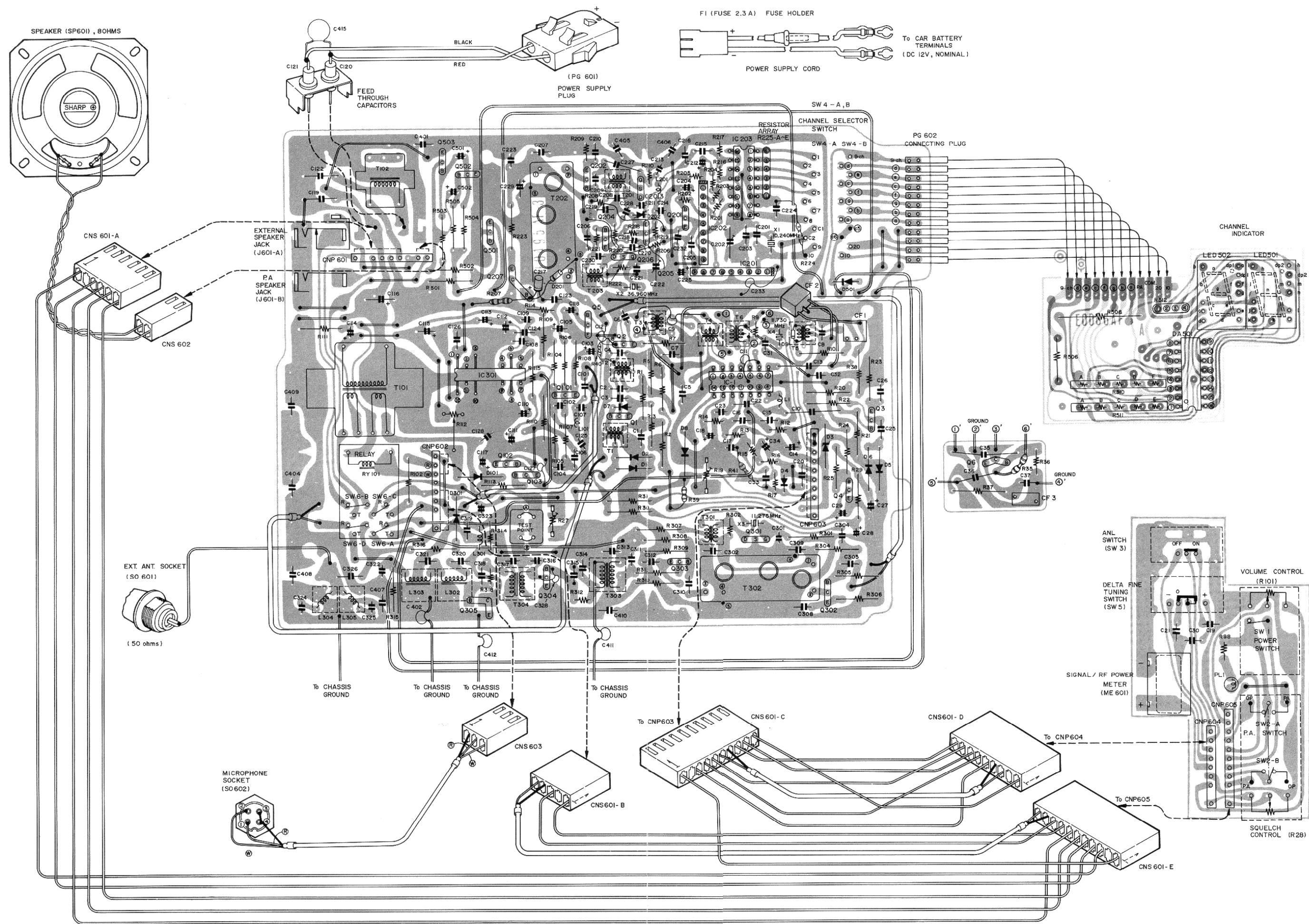
Figure 16 WIRING SIDE OF P.W. BOARD (OLD)
