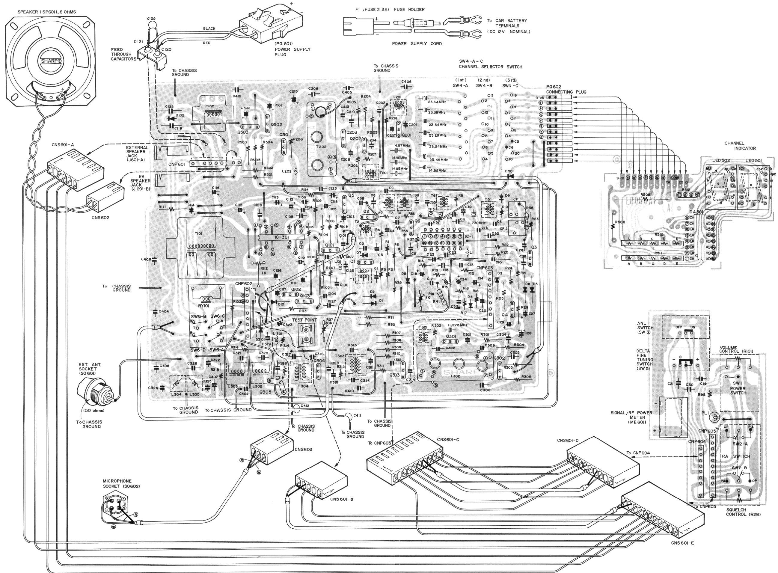
Figure 25 WIRING SIDE BOARD (P.W.B. NO. F0552AF)
