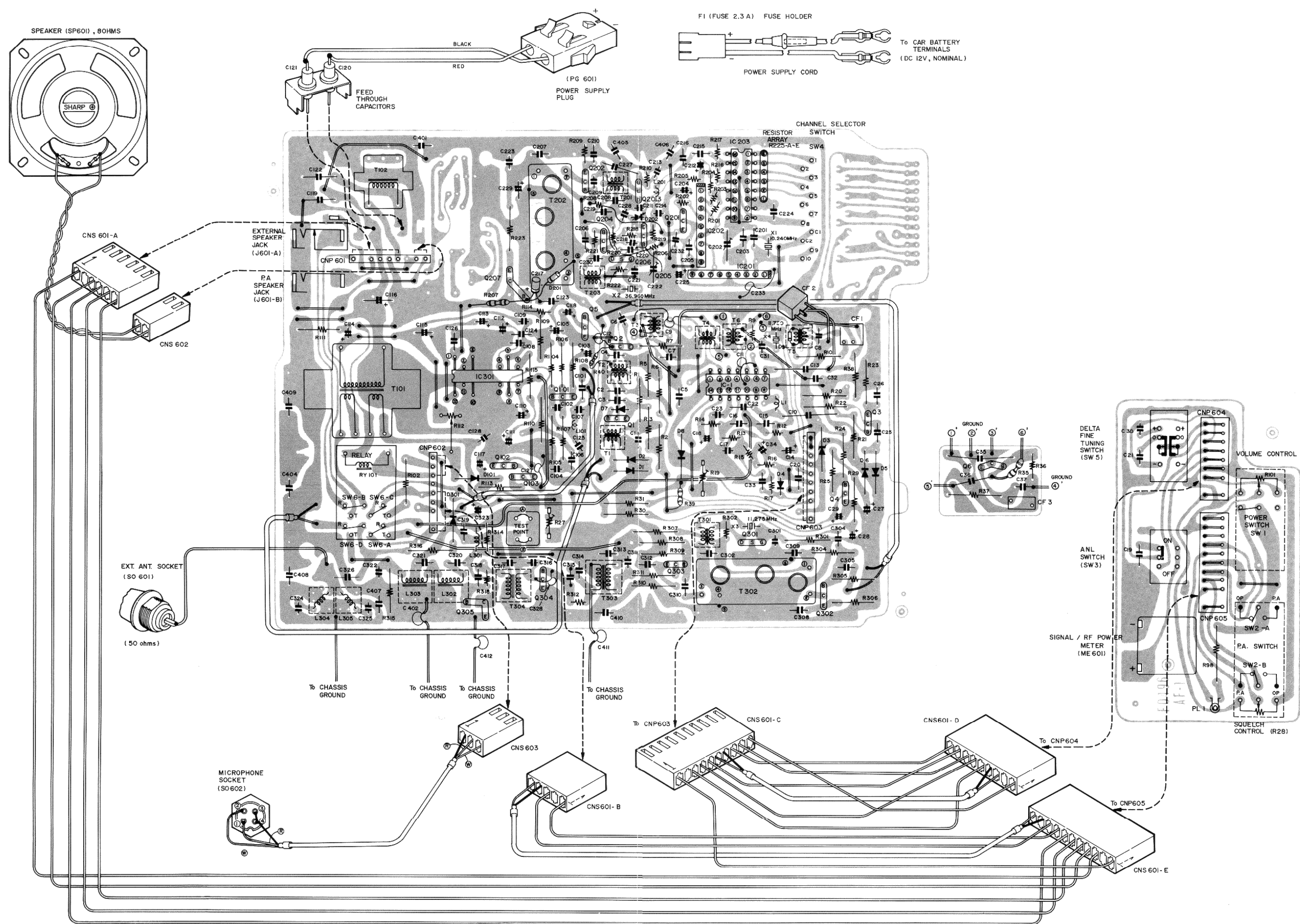
Figure 18 WIRING SIDE OF P.W. BOARD
