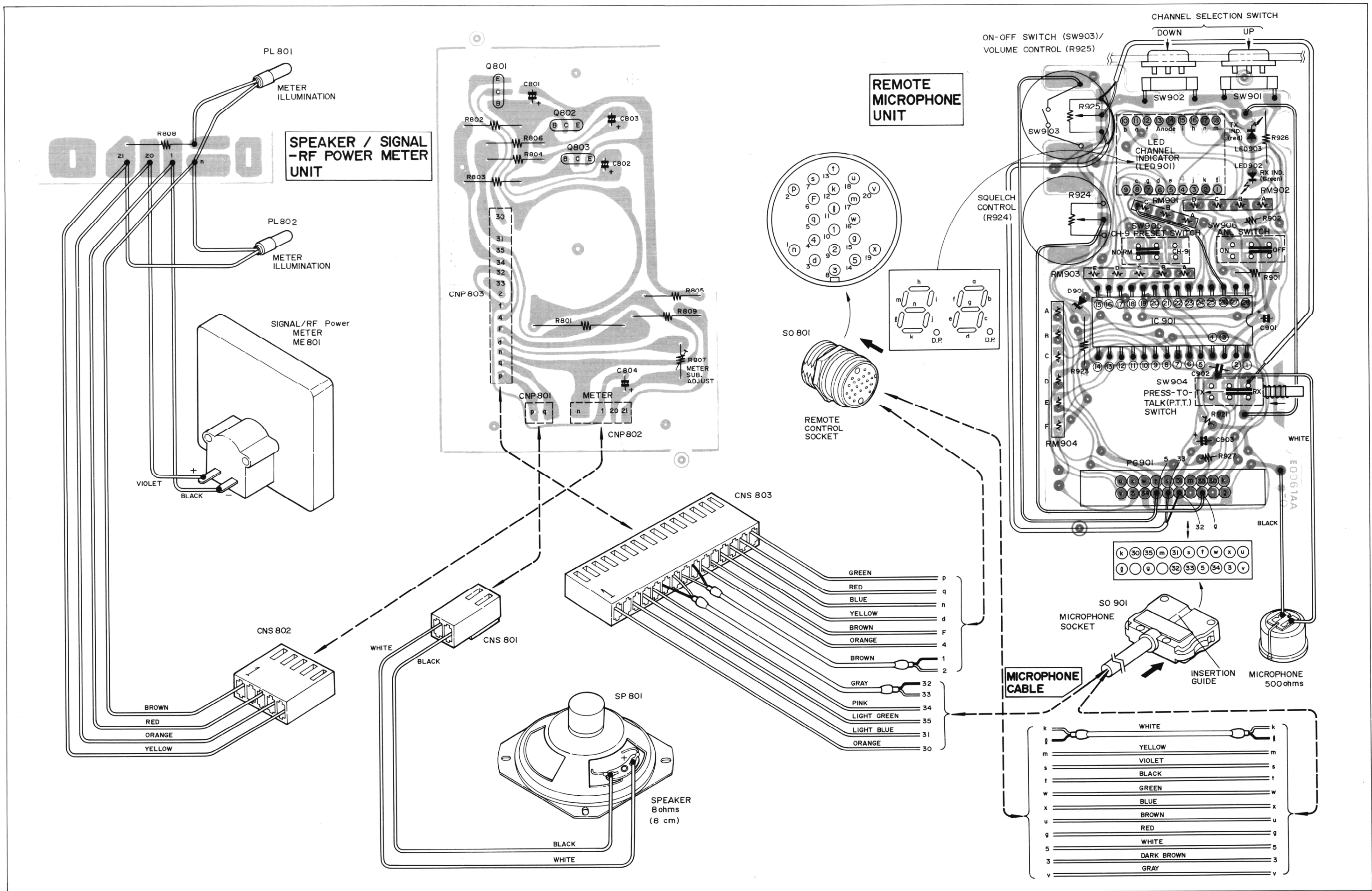
Figure 17 WIRING SIDE OF SPEAKER/SIGNAL-RF POWER METER UNIT AND REMOTE MICROPHONE UNIT P.W. BOARDS
