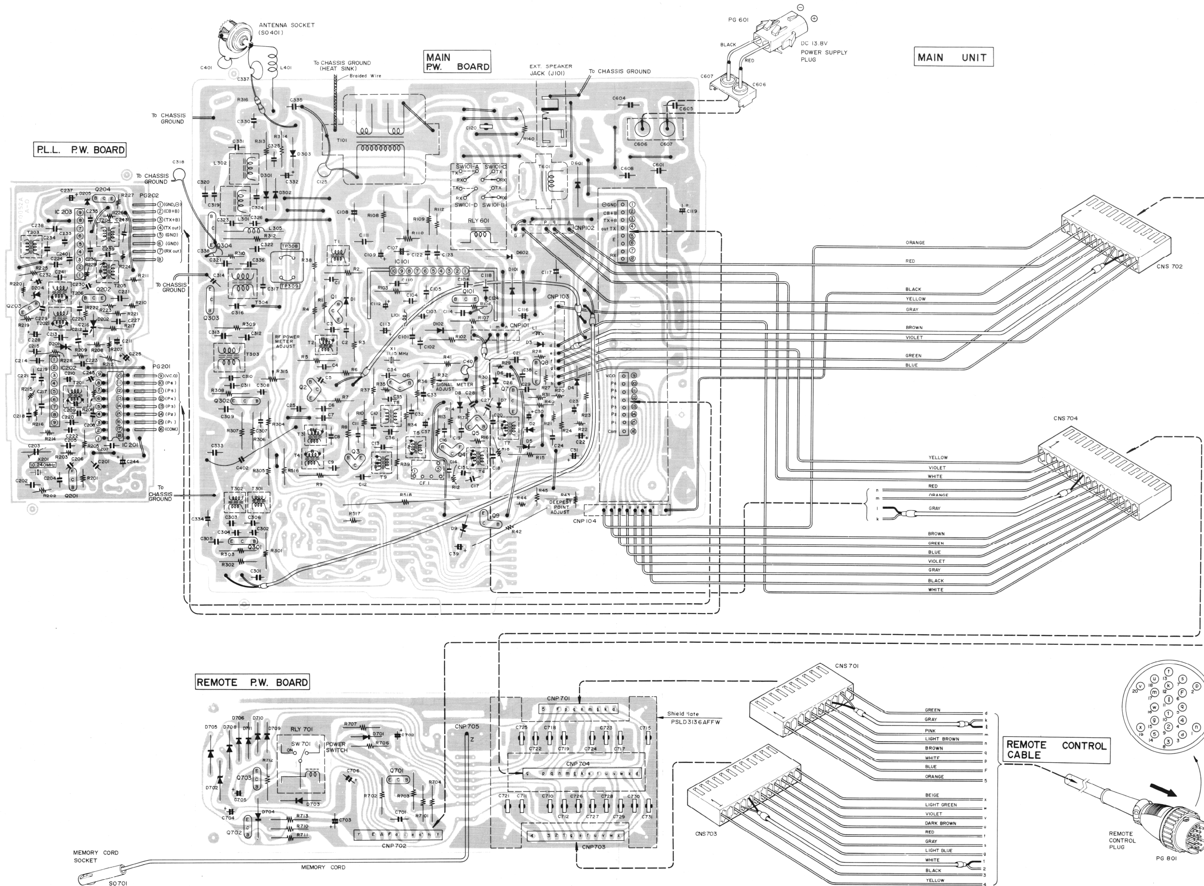
Figure 18 WIRING SIDE OF MAIN UNIT P.W. BOARDS
