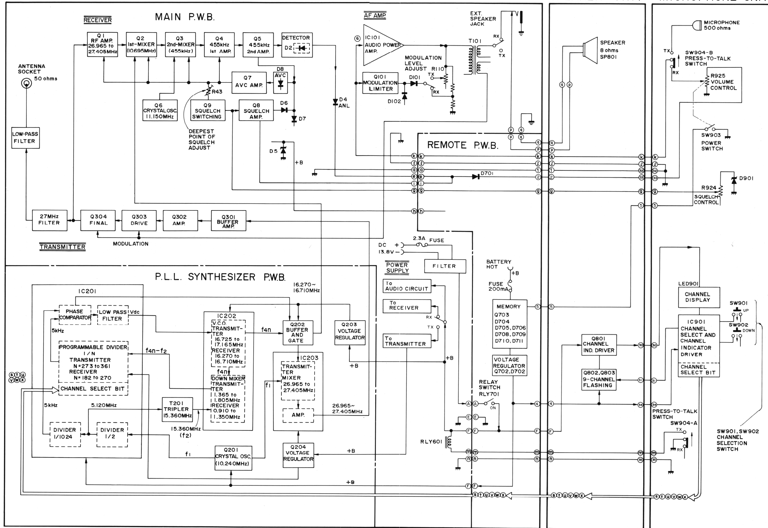
Figure 3 BLOCK DIAGRAM
