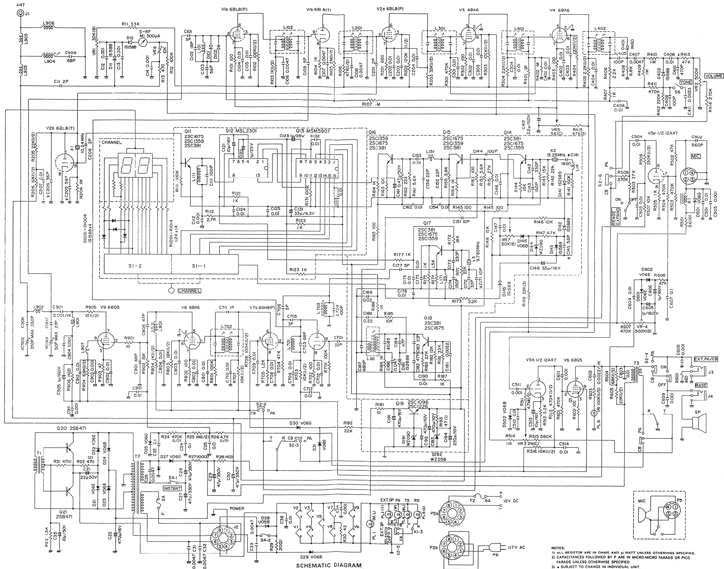
SCHEMATIC DIAGRAM
