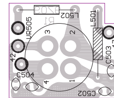
PCBX-0709R1 MIC SOCKET BOARD
