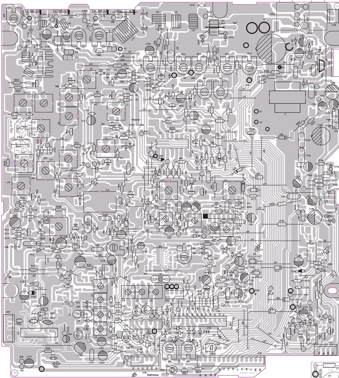
PCBX-0619R6 TOP LAYER MAGNUM S9 MASTER BOARD
