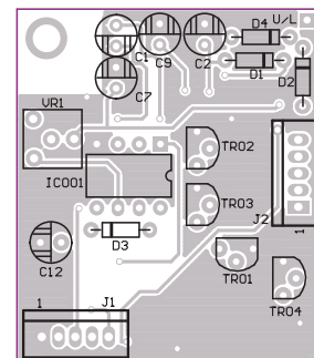
MAGNUM S9 VSWR CONTROL BOARD
