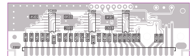
PCBX-0636R1 BOT LAYER MAGNUM S9 CHANNEL SWITCH BOARD
