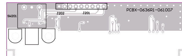
PCBX-0636R1 TOP LAYER MAGNUM S9 CHANNEL SWITCH BOARD
