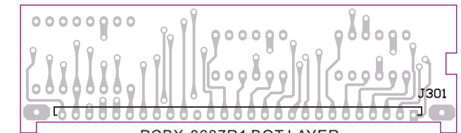
PCBX-0637R1 BOT LAYER MAGNUM S9 COUNTER DISPLAY BOARD
