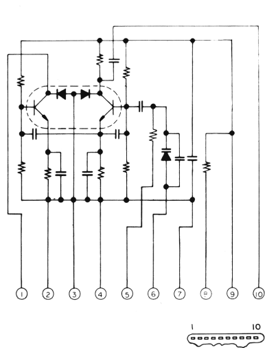
IC1 UHIC-070
