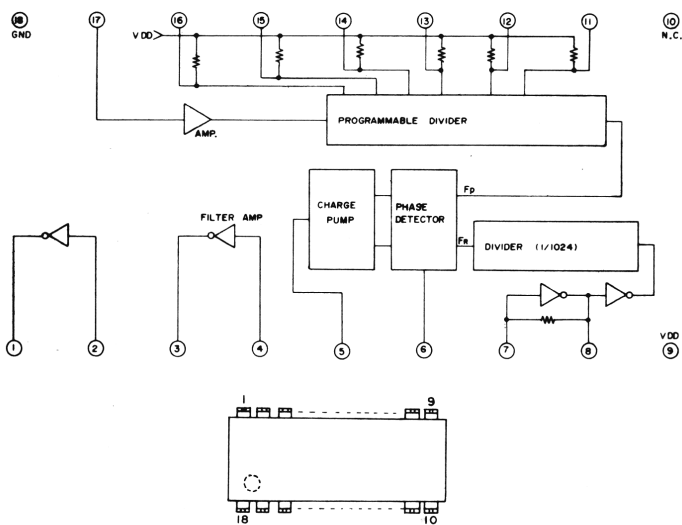
IC2 MB8734
