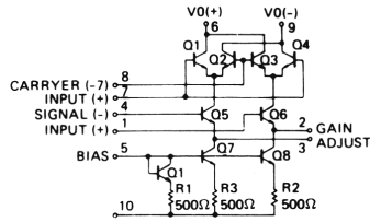
IC-2, MC1496N
