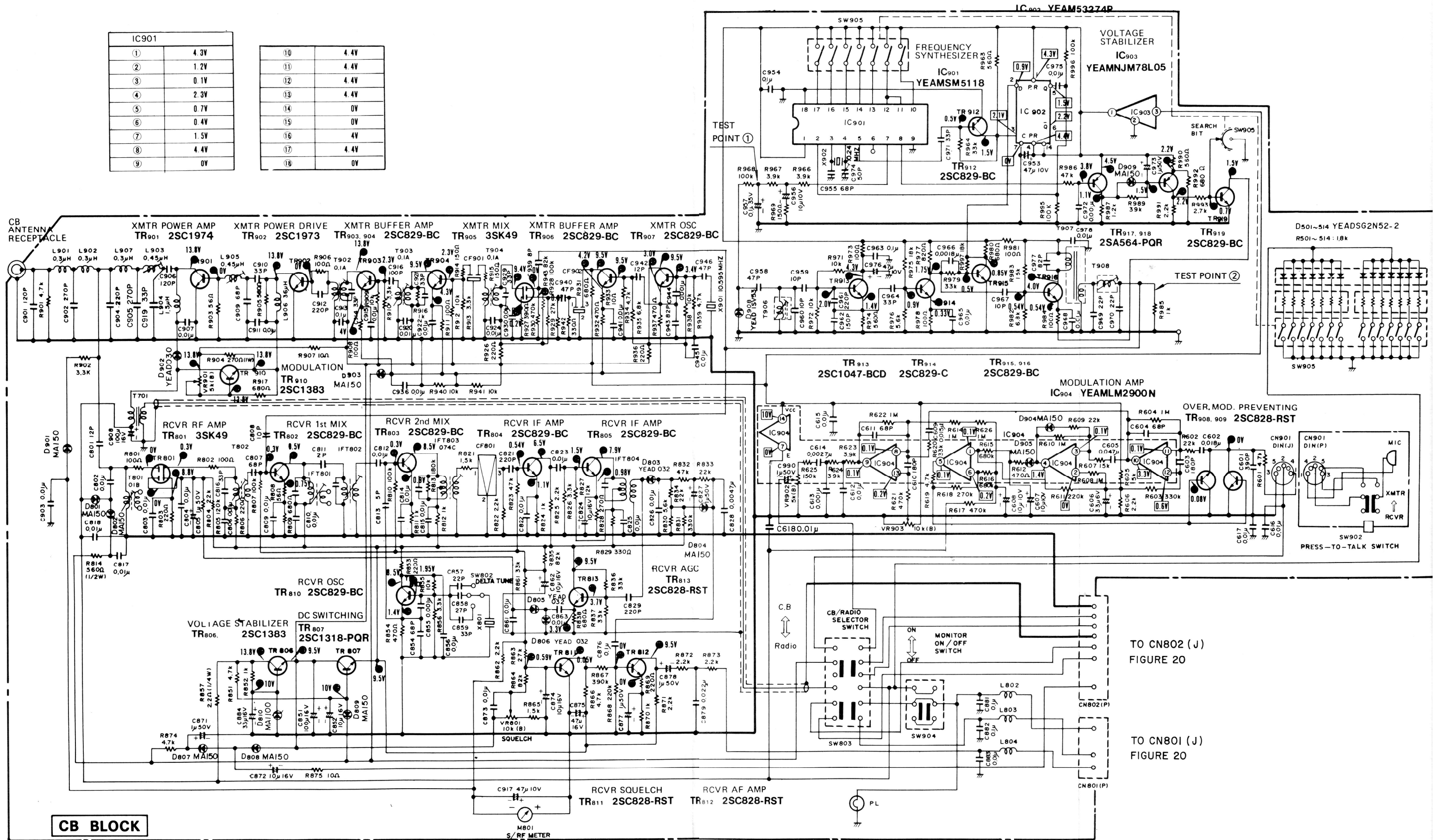
Figure 18. Schematic Diagram – CB Block – 14T410
