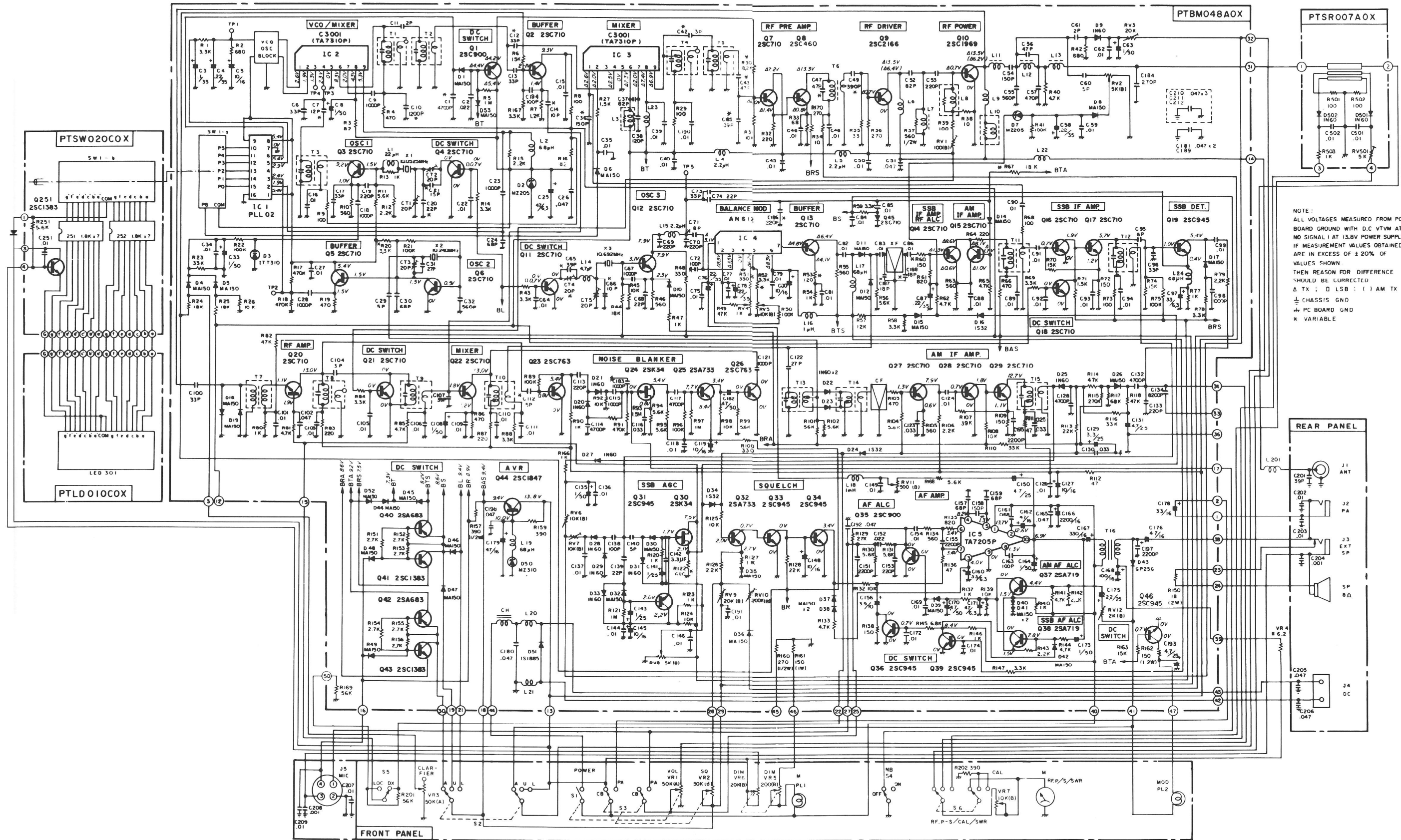
Figure 17 - Schematic Diagram - 14T302
