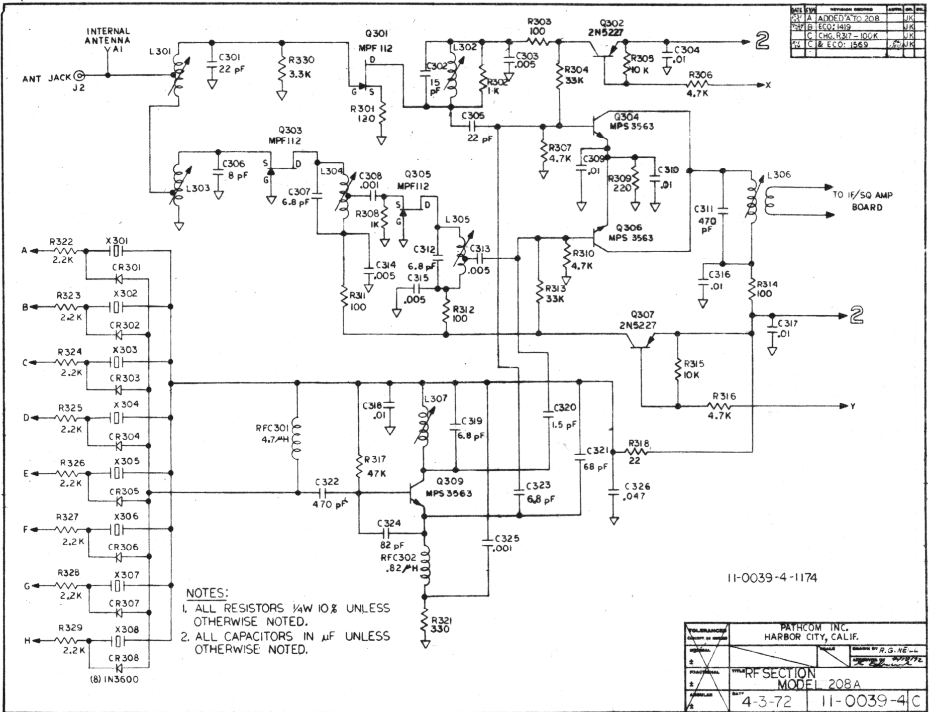
Figure 6-9. VHF/RF Circuit for SCAN 208A
