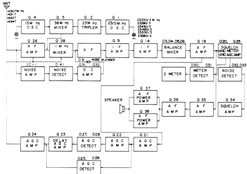
BLOCK DIAGRAM C
