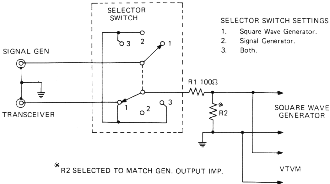
FIGURE 3. NOISE SILENSER ADJ TEST FIXTURE
