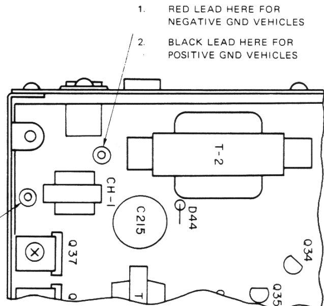
TELSAT SSB-50 INTERNAL VIEW
