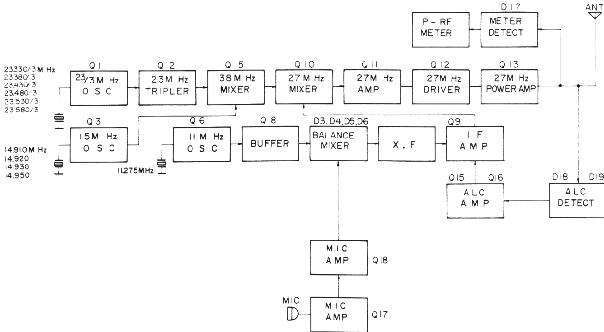
BLOCK DIAGRAM E
