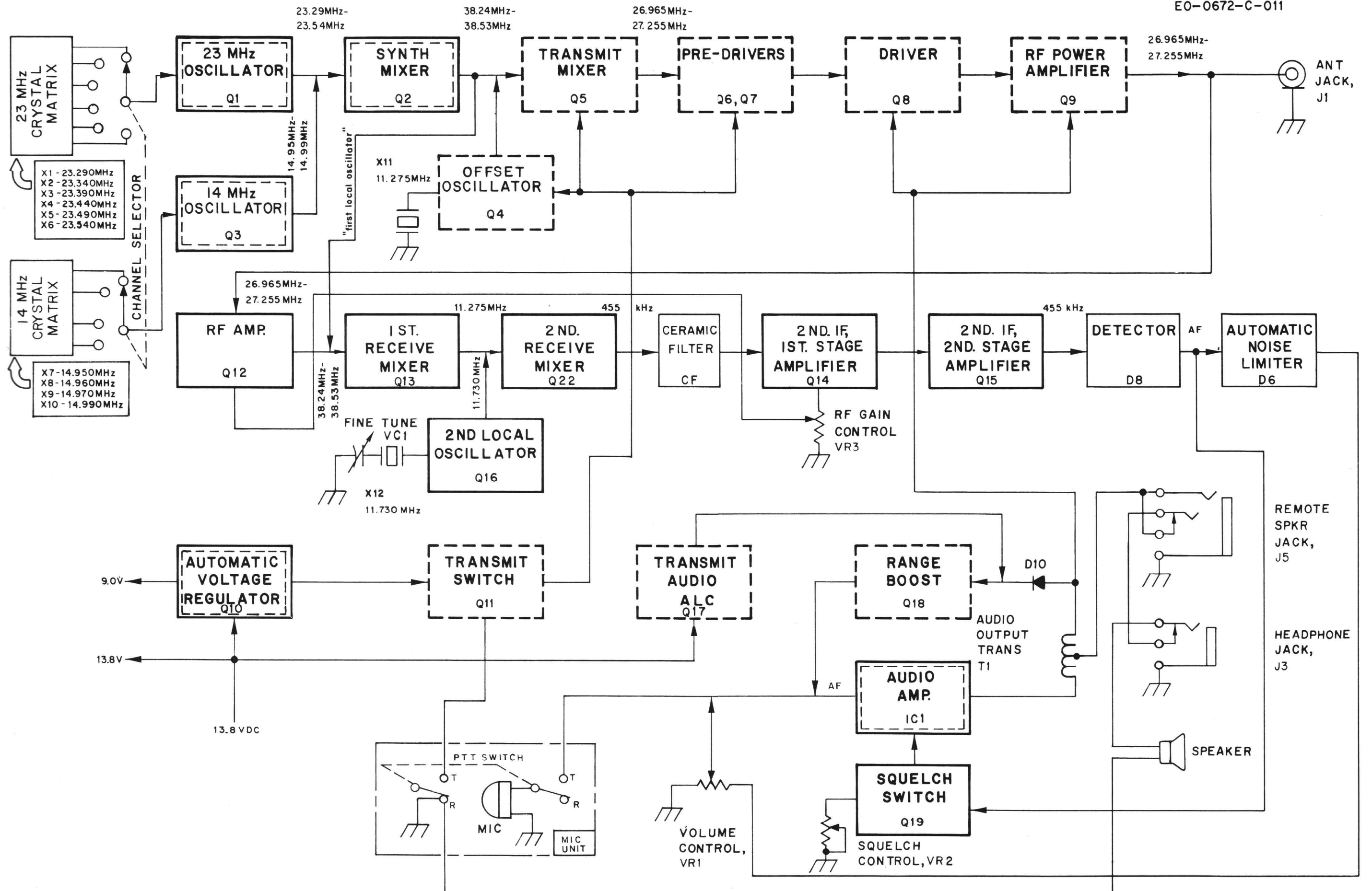
Figure 2-1. Block Diagram
