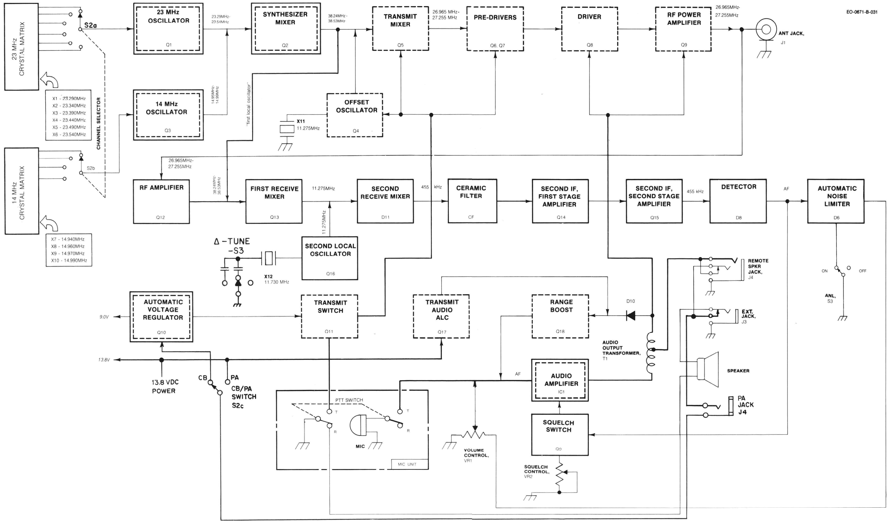
Figure 2-1. Block Diagram, 671B
