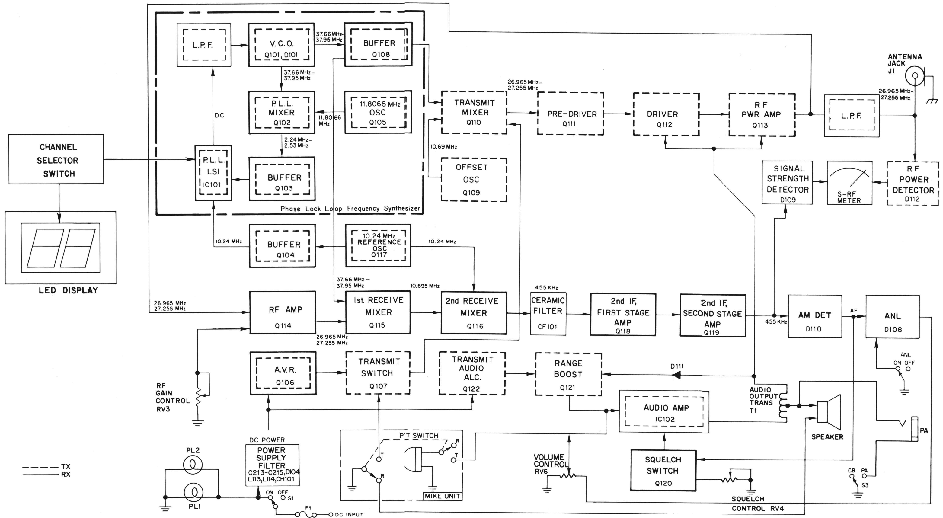
Figure 2-2. Block Diagram, Model 2702A
