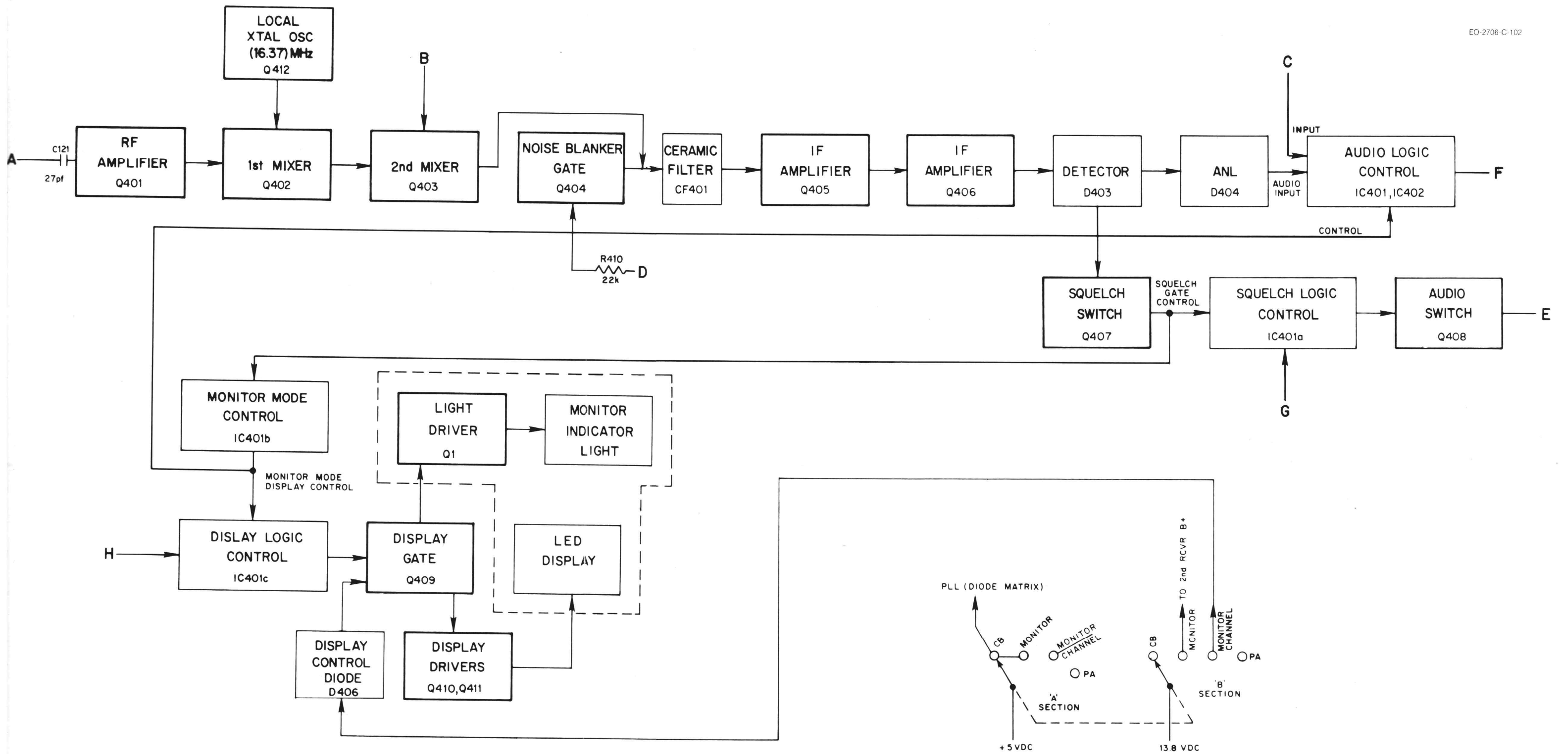
Figure 2-3. Block Diagram, Monitor Receiver
