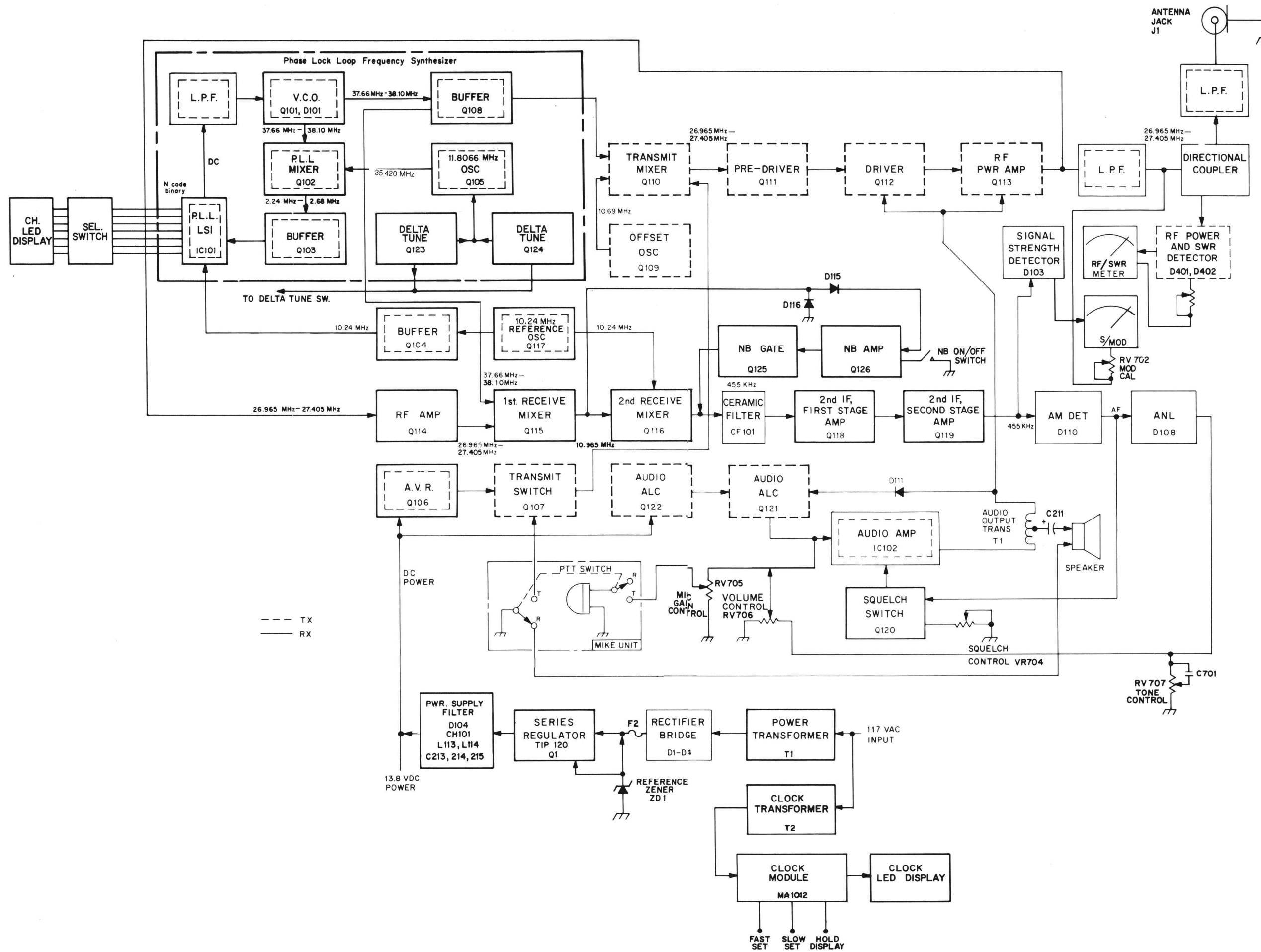
Figure 2-3. Block Diagram Model 3114
