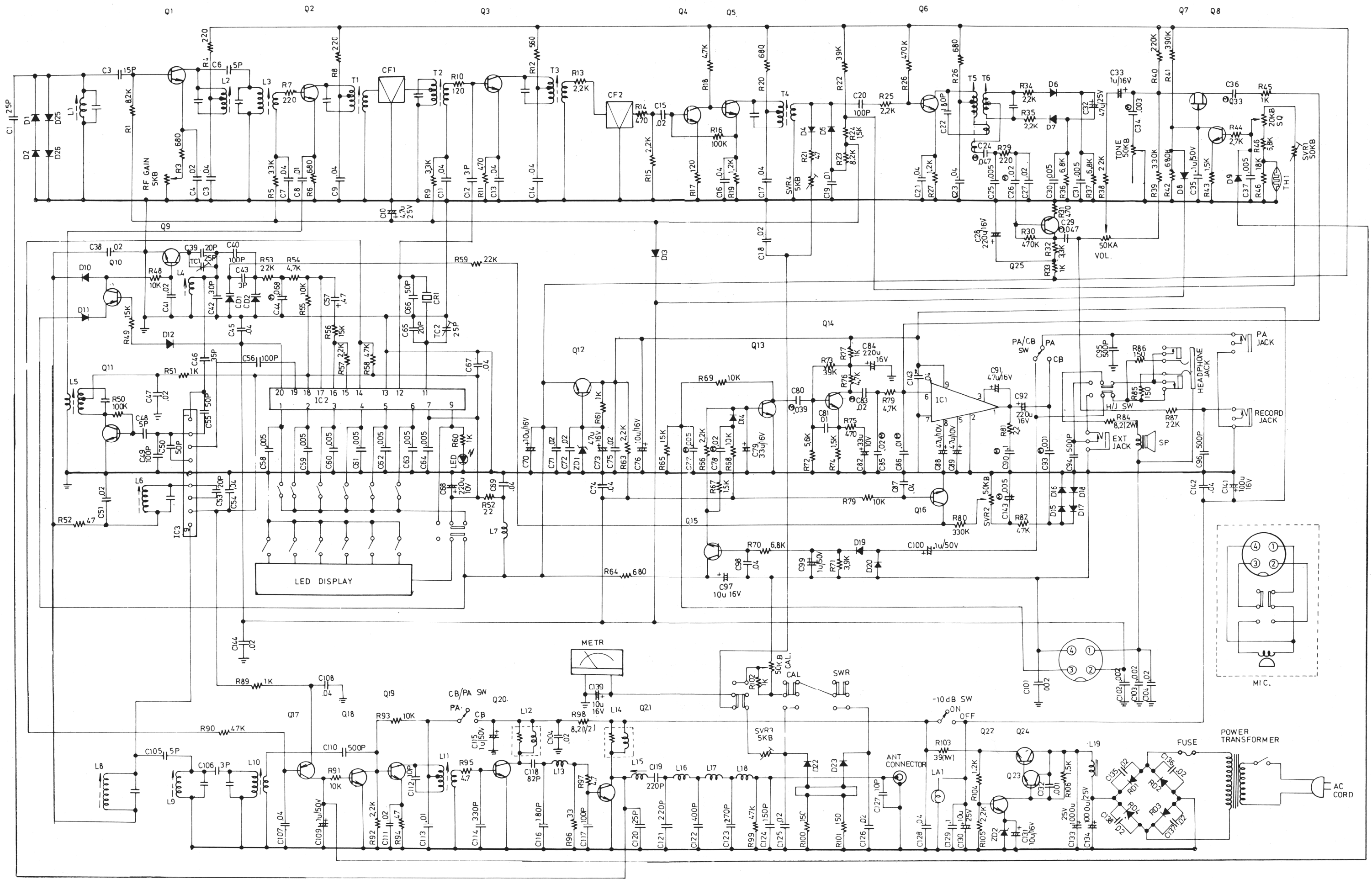
CIRCUIT DIAGRAM
