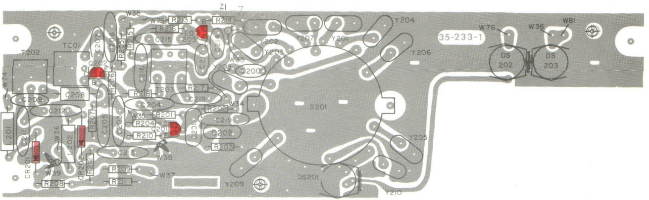
FREQUENCY SYNTHESIZER BOARD SOLDER SIDE VIEW
