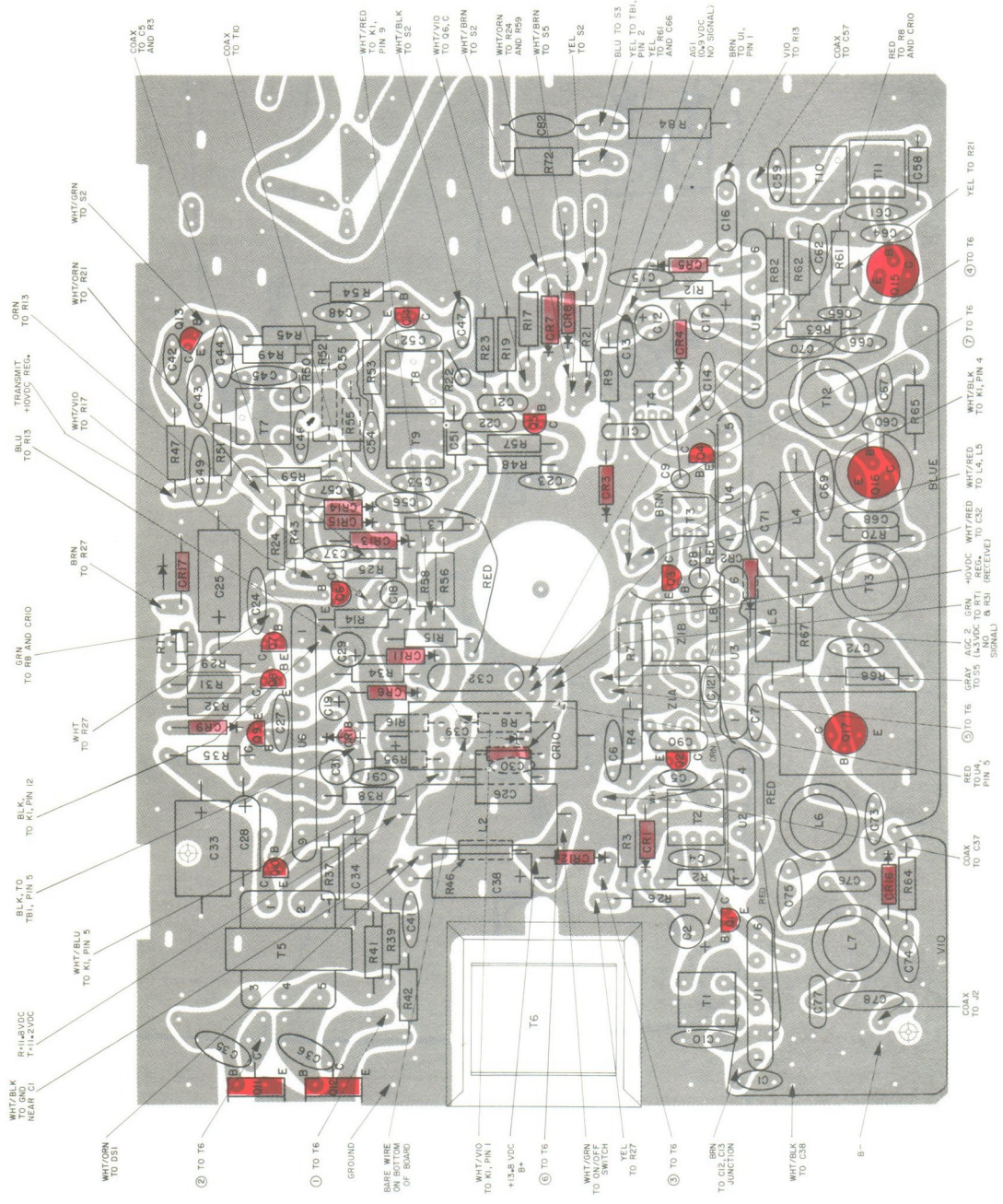
COMPONENTS LAYOUT (SOLDER SIDE VIEW)
