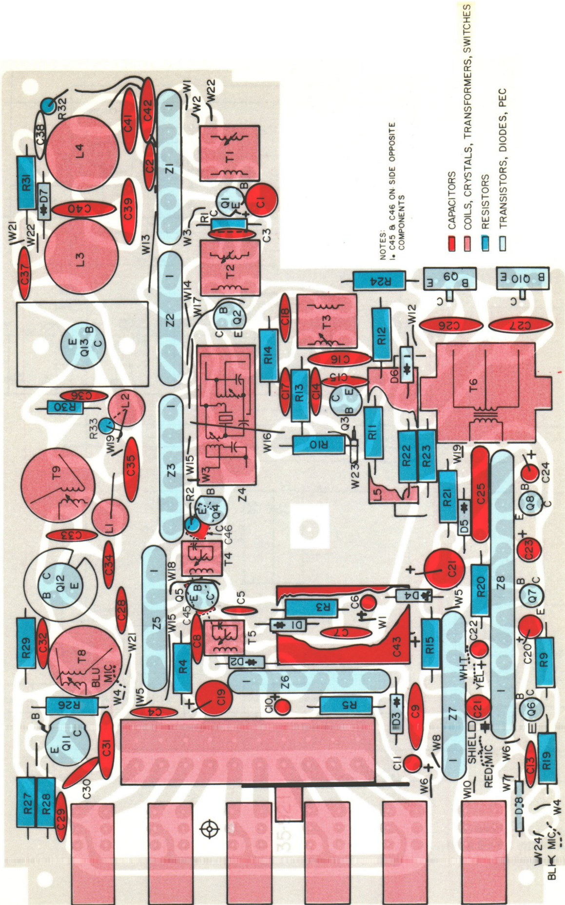
MESSENGER 125 PRINTED CIRCUIT BOARD
