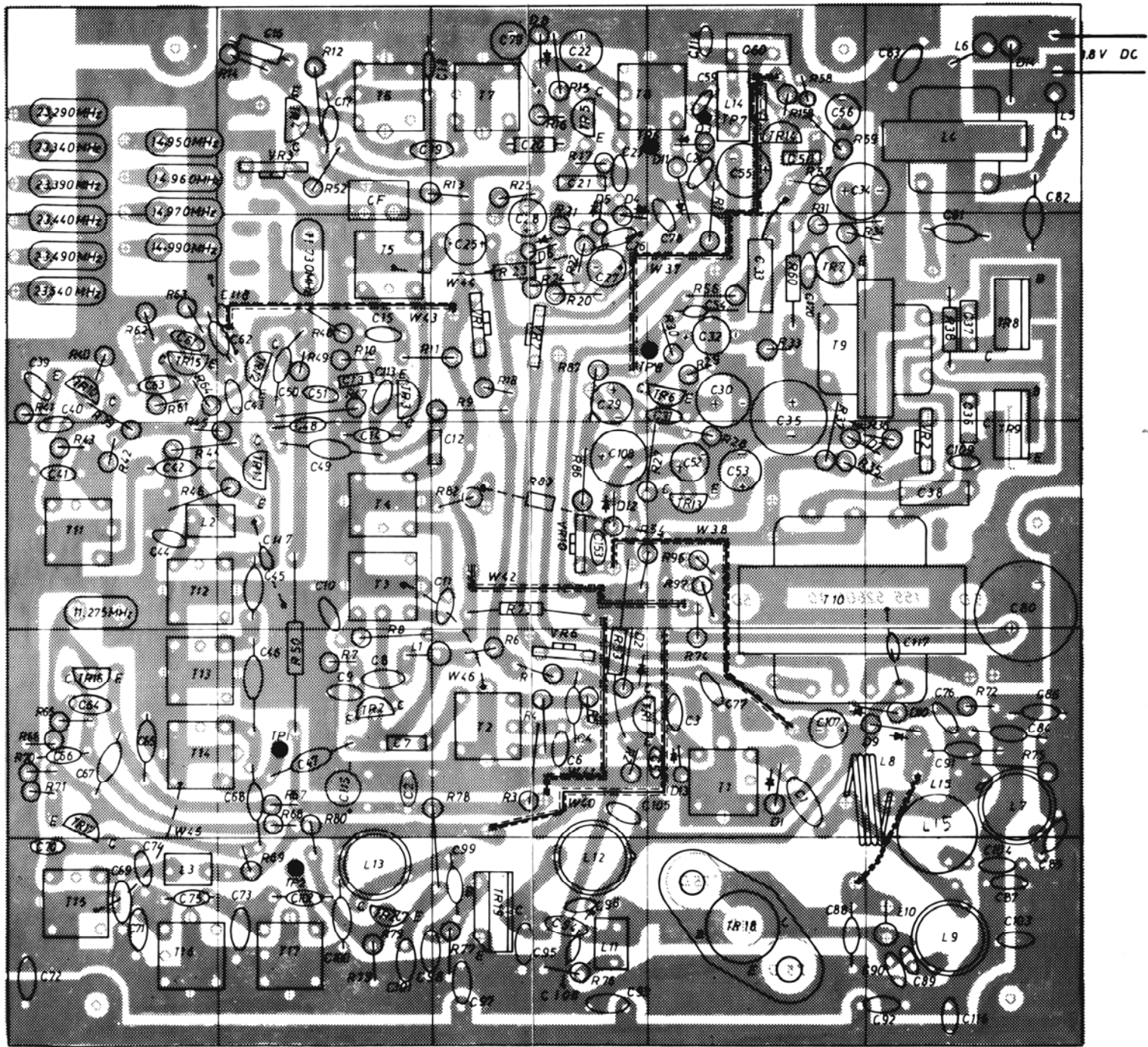
FIGURE 5, COMPONENT LOCATION
