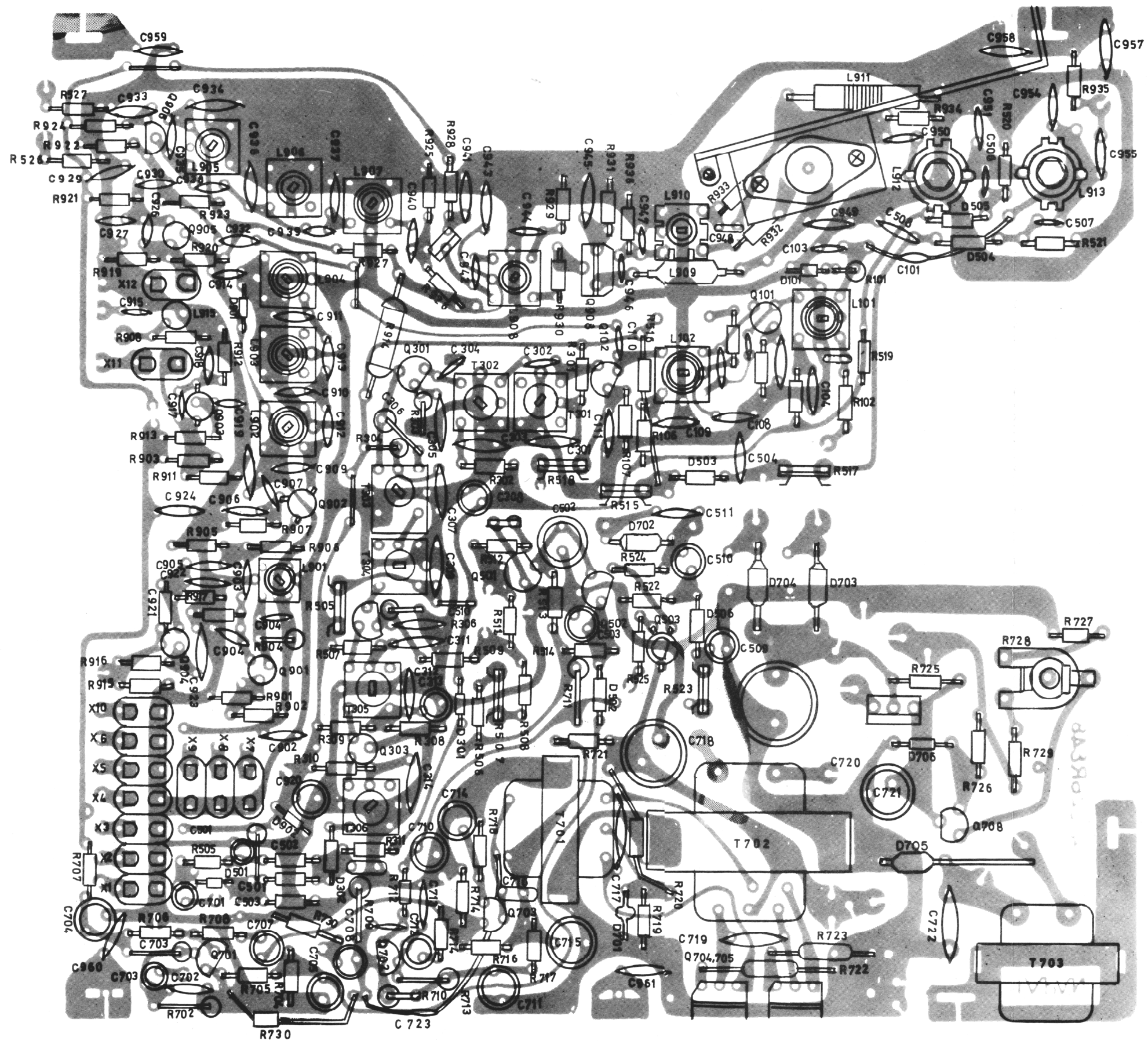
FIGURE 10, PRINTED CIRCUIT BOARD, COMPONENT LOCATION
