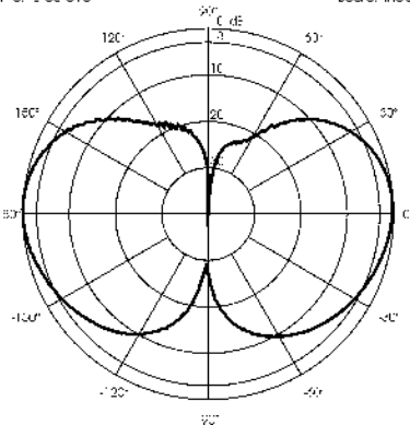
TYPICAL RADIATION PATTERN in E-plane at 435 MHz File: F-03-010 Scale: linear
