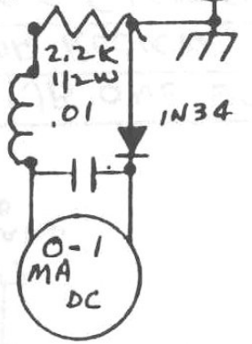
Field strength meter
