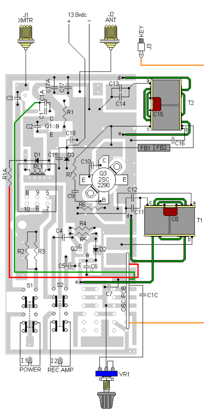
CW Transmitter Before Conversion
