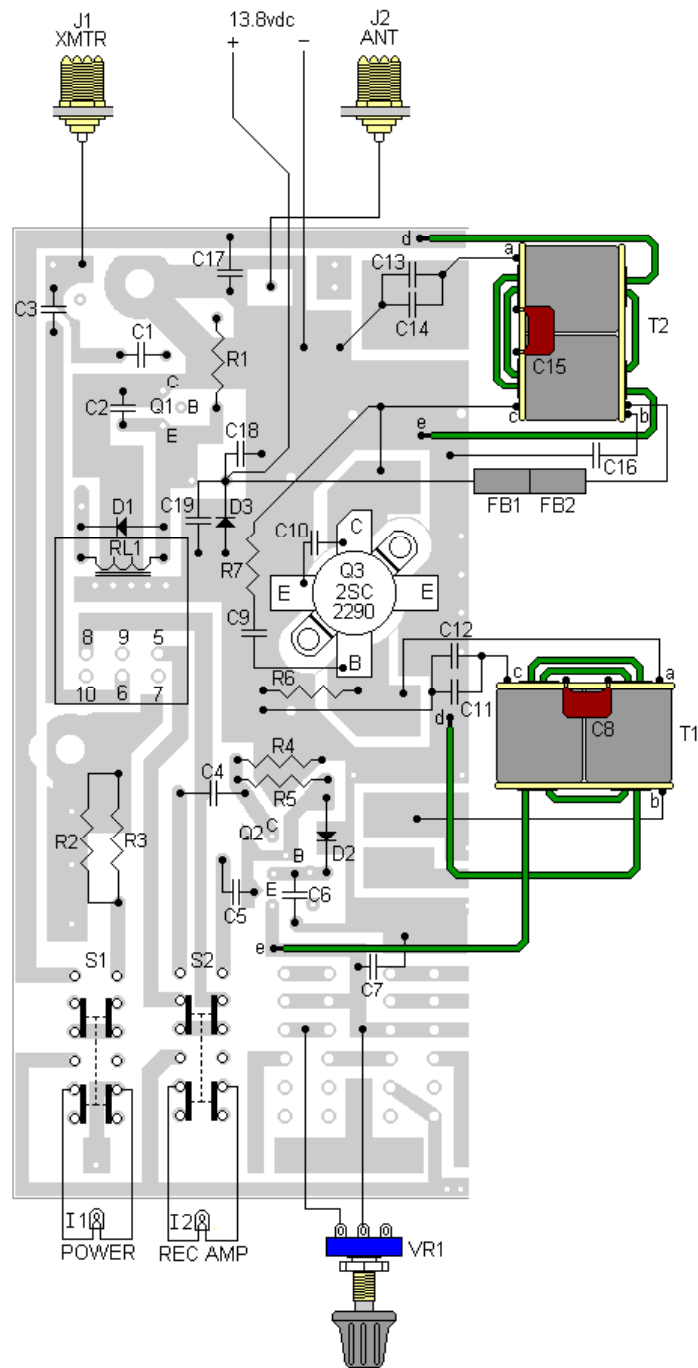
Amp After Conversion
