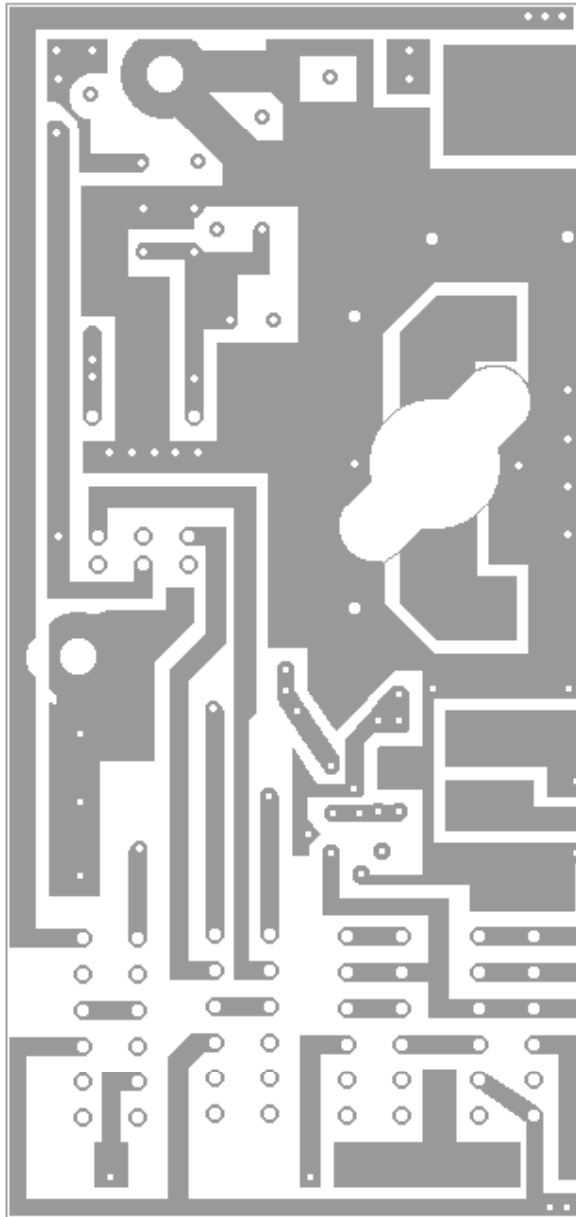
Board E Top View
