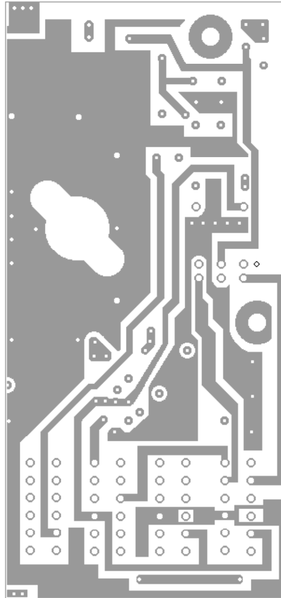
Board E Bottom View
