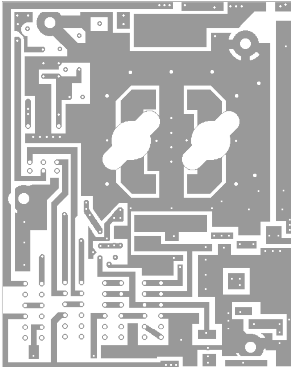
Board A Top View Used in the Following DX250 DX350 DX400 DX 500 Front PCB
