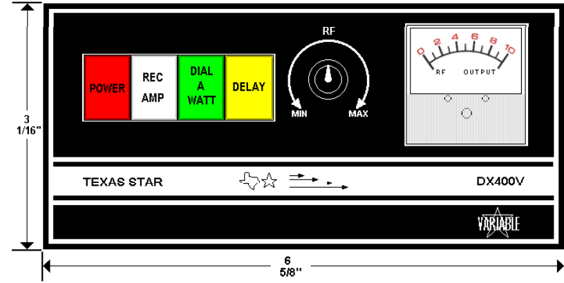
DX400V Front View
