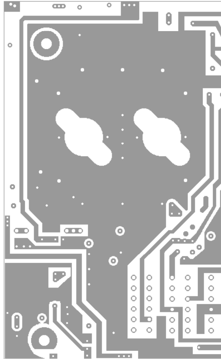
Board D Bottom View
