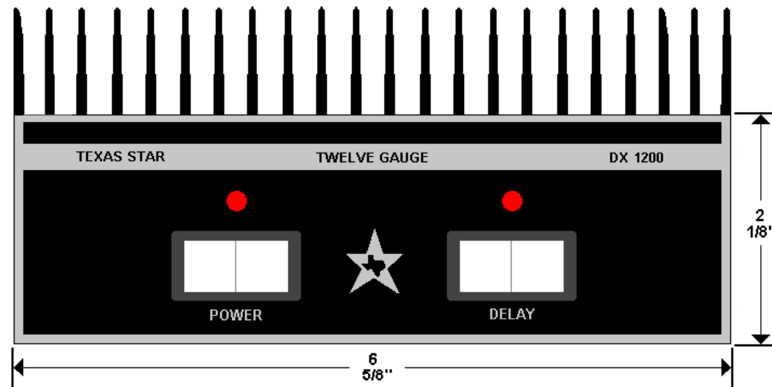
DX1200 FRONT VIEW
