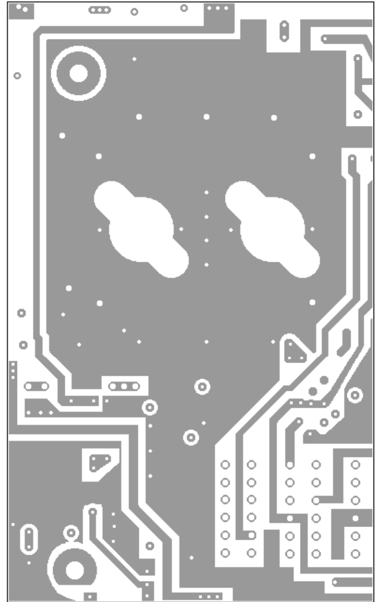
Amp PCB Board #1 - #4
