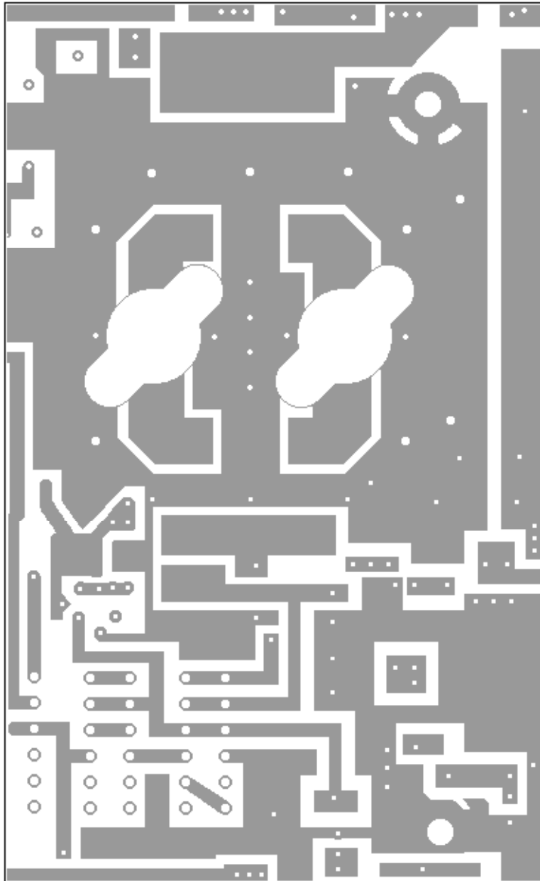
Amp PCB Board #1 - #4 Top View
