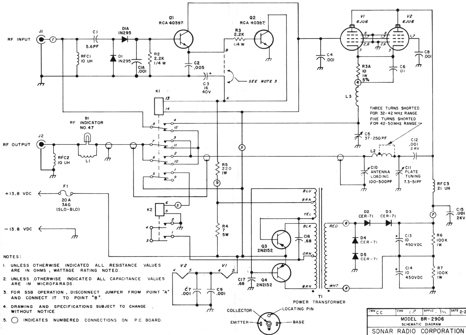
TRANSISTOR BASE DIAGRAM Q3,Q4
