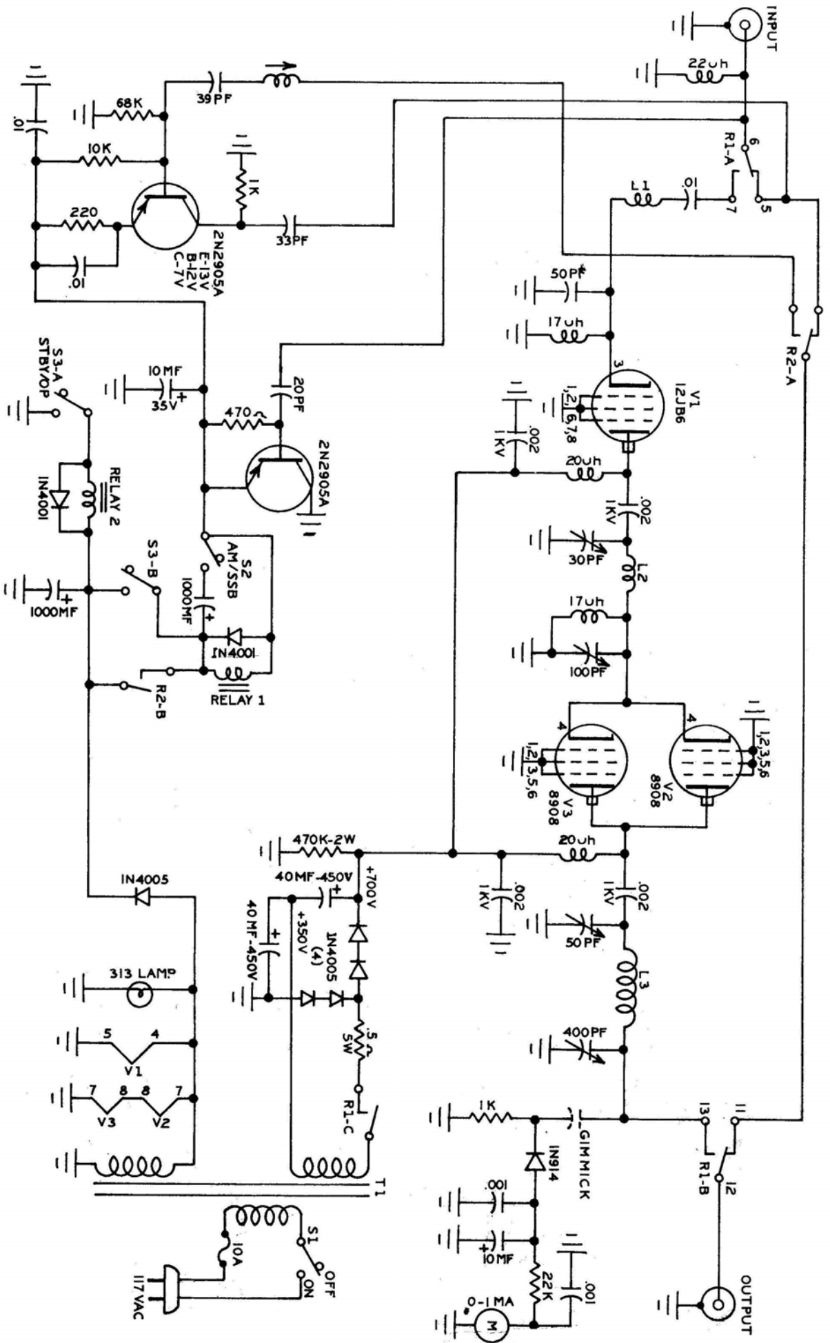
SCHEMATIC DIAGRAM - PALOMAR MODEL 200 BI-LINEAR AMPLIFIER PALOMAR INSTRUMENT CO. - Escondido, Calif. 7-13-71
