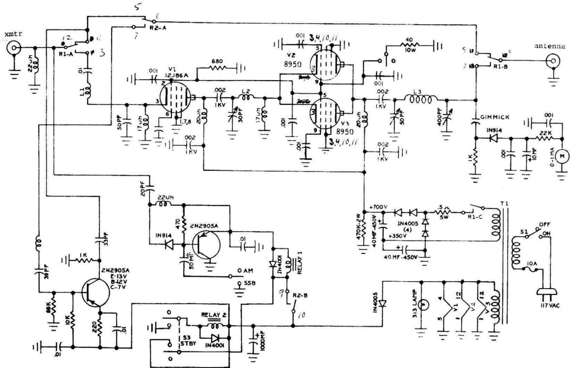
SCHEMATIC DIAGRAM--MODEL 160 BI-LINEAR AMPLIFIER PALOMAR ELECTRONICS CORP. ESCONDIDO, CA 92025
