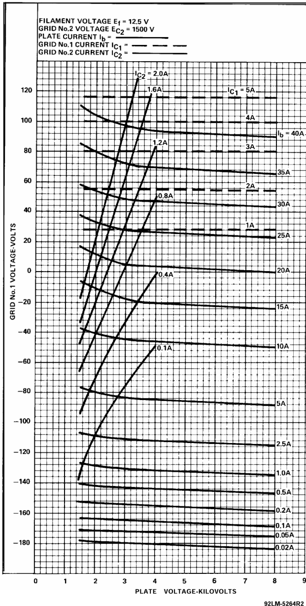
Figure 5 - Typical Constant Current Characteristics
