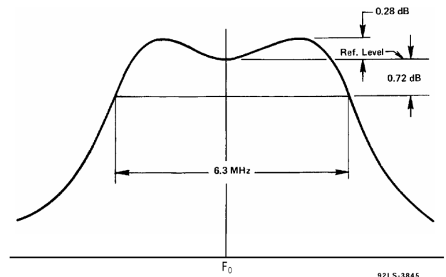
Figure 2 - Bandwidth Characteristics
