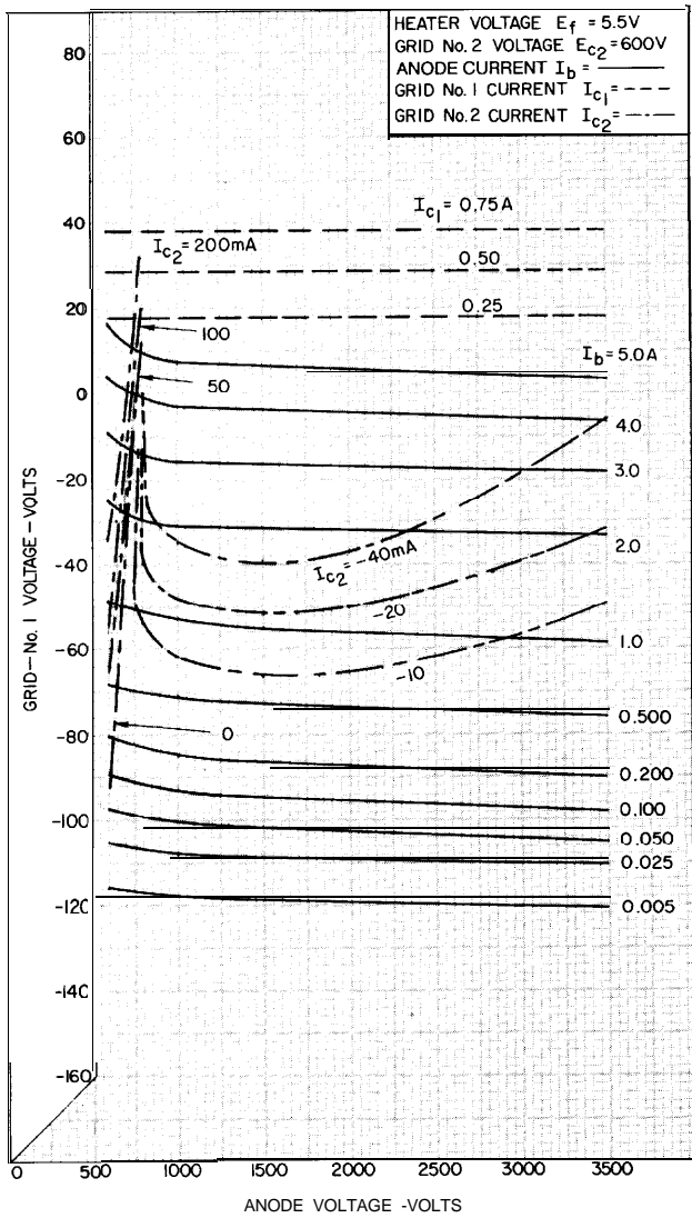
Figure 2 - Typical Constant Current Characteristics ( E_{c2} = 600 V )
